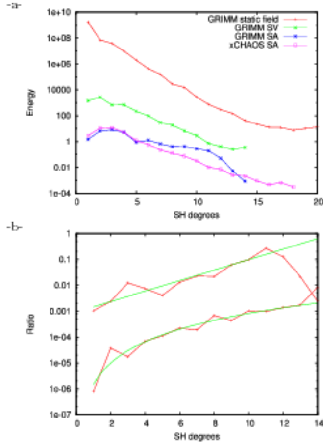
Figure 3. -a- Power spectra of the core field, its secular variation and secular acceleration for year 2003.25 at Earth's reference radius. The acceleration power spectrum is compared with xCHAOS secular acceleration spectrum for the same date. -b- degree by degree ratio of the power in secular variation to the power in core field (bottom curve) and to the power in secular acceleration to that in secular variation (top curve). Also shown are power law and exponential law fits.
