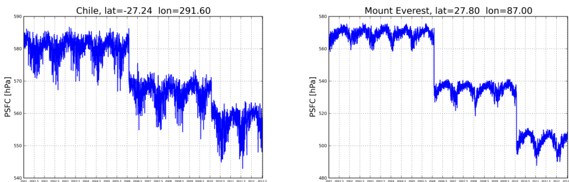
Figure 3-3: 6-hourly surface pressure variation between January 2001 and June 2012 at a location in Chile (left) and over Mount Everest (right). Two discontinuities are visible in January 2006 and January 2010.
