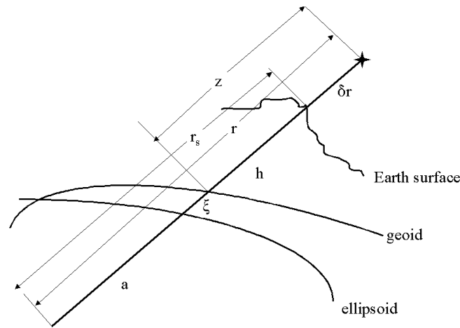
Figure 3-2: Radial component r used in vertical integration
